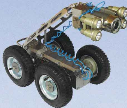
P-200 CCTV Robotic System CCTV inspection for pipelines from 150 mm to 1800 mm in diameter
